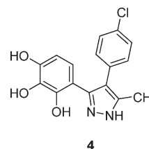
Figure 2. Chemical structure of screening hit 4 .
