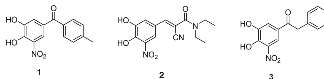
Figure 1. Chemical structures of tolcapone 1 , entacapone 2 , and nebicapone 3 .
